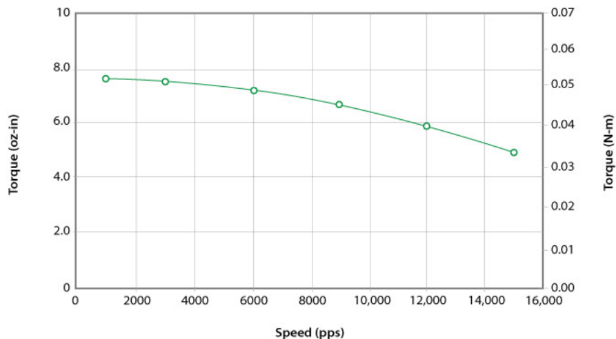
3809X-51 24VDC, 0.6 Amps/Phase, Bipolar, 1/2 Stepping
